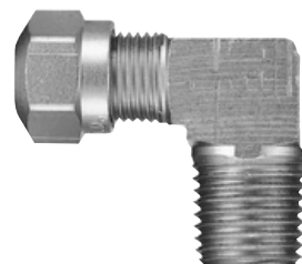
84283 Male Elbow 90° 1/4 Tube x 1/4 NPT
