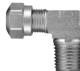
84285 Male Elbow 90° 3/8 Tube x 3/8 NPT
