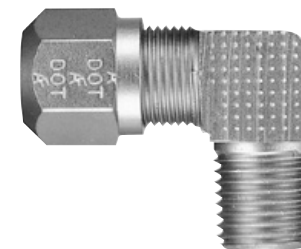
84284 Male Elbow 90° 3/8 Tube x 1/4 NPT
